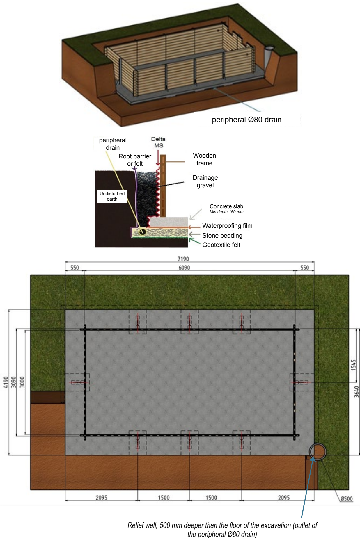
Figure 1 – Drainage system installation diagram
