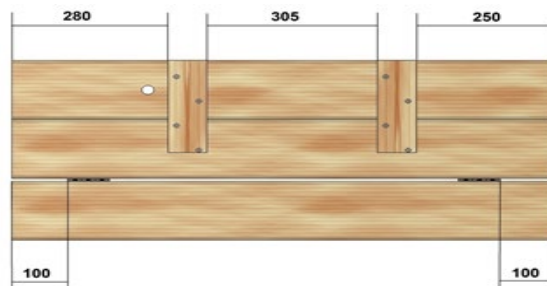
Figure 64 – Assembly of the duckboarding
