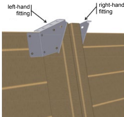
Mounting the fittings on top of the supporting brace
