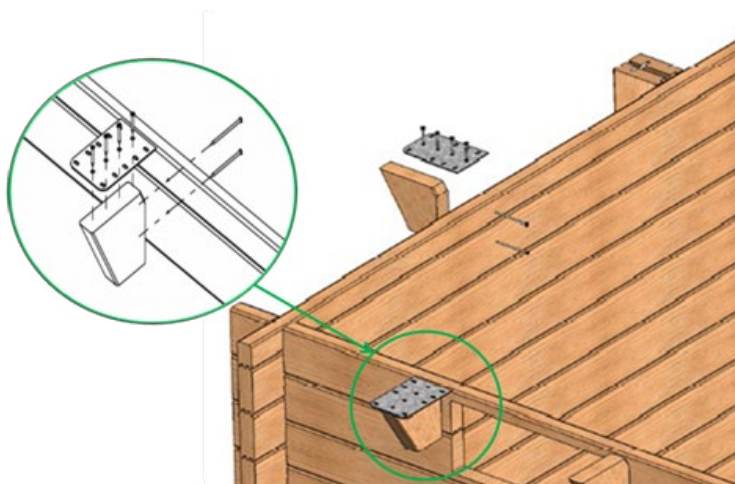
Figure 13 – Fastening metallic plates to the wooden brackets
