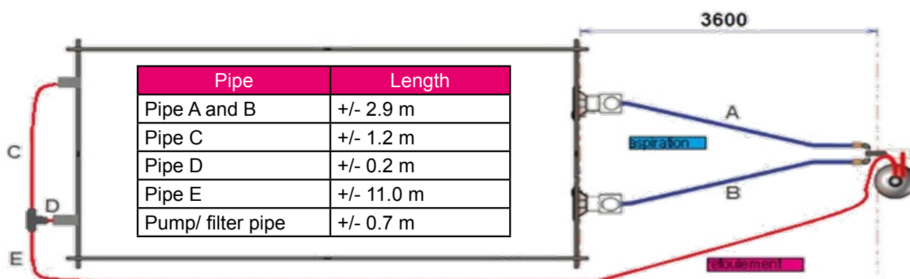
Figure 24 – Positions of the various pipes
