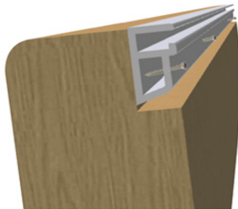
Figure 26 – Installing the liner locking track
