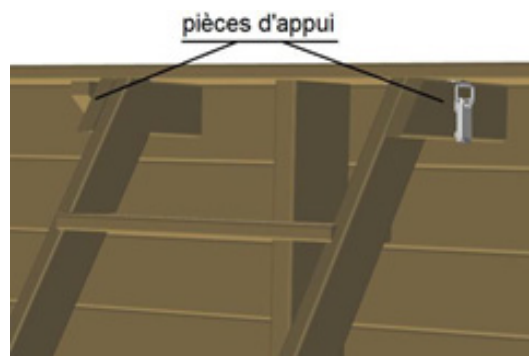
Figure 37 – Assembling the wooden access ladder
