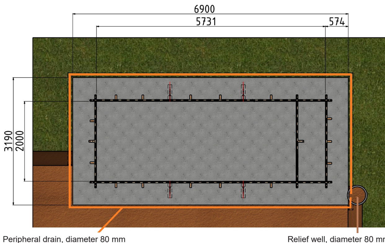
Figure 1 – Drainage system installation diagram
