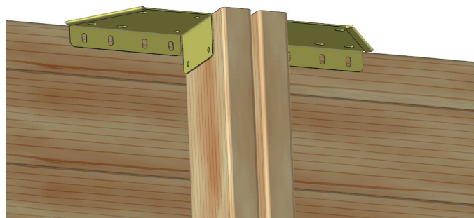
Figure 18 – Fastening metallic support brackets to the top of the supporting braces
